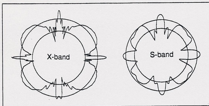
Above left: Fig. 4. RCS plot of the Davis Echomaster in the double catch rain position with 0^\circ heel.
