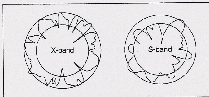
Right: Fig. 6. RCS plot of the Firdell Blipper 210-5 with 0^\circ heel. Below left: Fig. 7. RCS plot of the Radar Flag (draped) with 0^\circ heel. Below right: Fig. 8. RCS plot of the 2" radius Mobri with 20^\circ heel.
