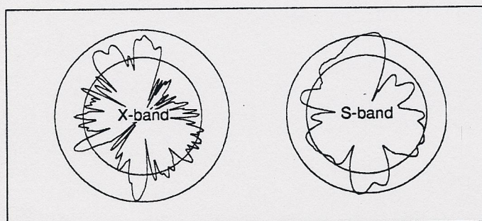
Right: Fig. 6. RCS plot of the Firdell Blipper 210-5 with 0^\circ heel. Below left: Fig. 7. RCS plot of the Radar Flag (draped) with 0^\circ heel. Below right: Fig. 8. RCS plot of the 2" radius Mobri with 20^\circ heel.
