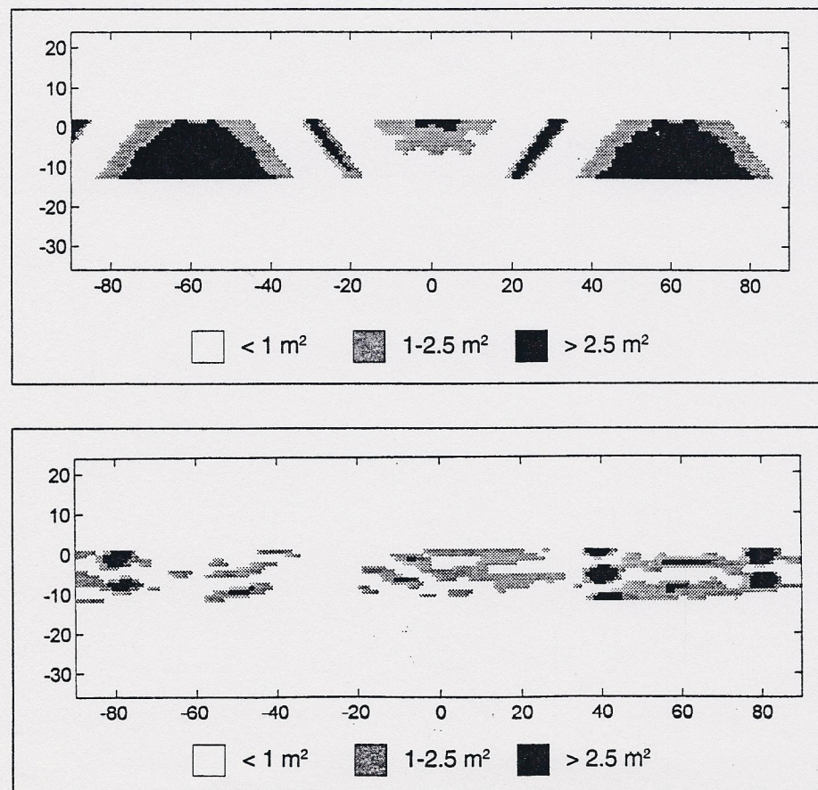
Below top: Fig. 9. Target Pattern Map (TPM) of the Davis Echomaster in the catch-rain position. Below bottom: Fig. 10. Target Pattern Map (TPM) of the Firdell Blipper 210-5.
