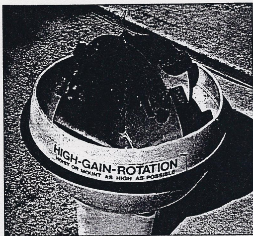
Above left: The High Gain Rotation (about $90) is a plastic sphere with a gimbaled quadrahedral reflector inside. In this photo, it is shown cut open. Above right: The Cyclops 1 (the smallest of three models) sells for about $300 and has a sturdy masthead mount.
